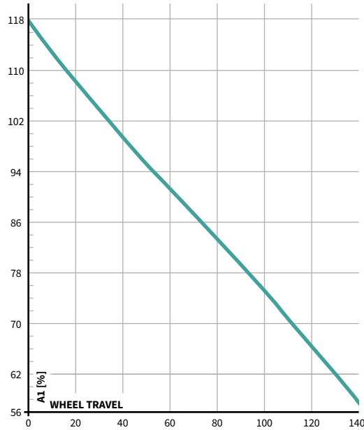
ANTI-SQUAT (32/28)
