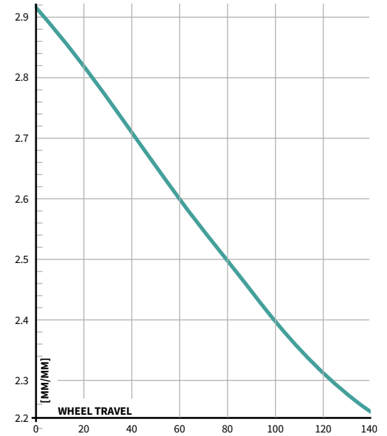
LEVERAGE RATIO
