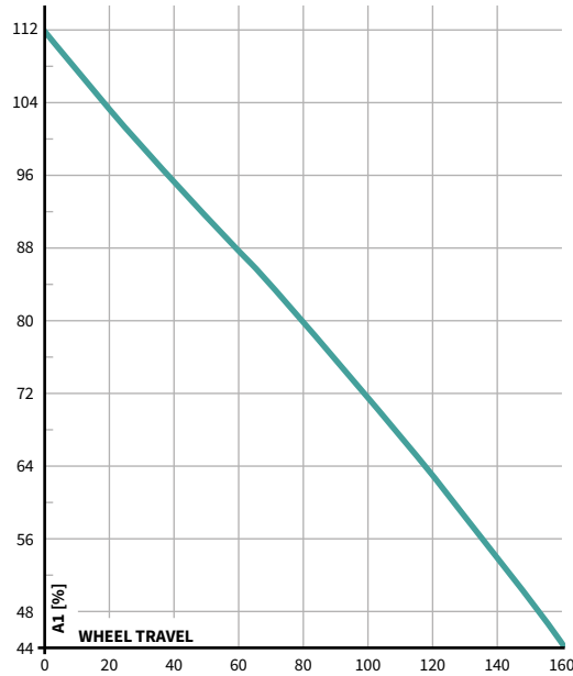
ANTI-SQUAT (34/36)
