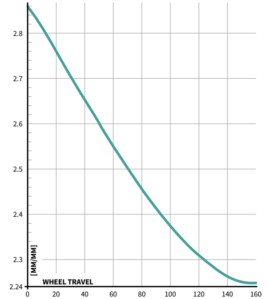
LEVERAGE RATIO
